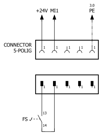
FOOT SWITCH
