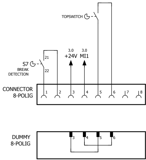
PLC - TOPSWITCH
